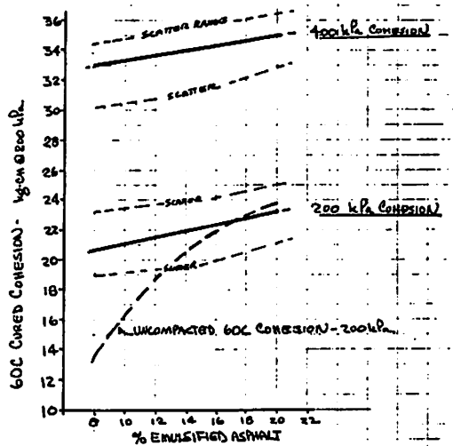
EXAMPLE 3. COHESION OF 100GRAM SPECIMENS COMPACTED @ 2 TONS, 2 MINUTES @ 60C.
