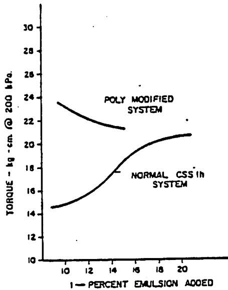
EXAMPLE 18. 140°F CURED COHESION
