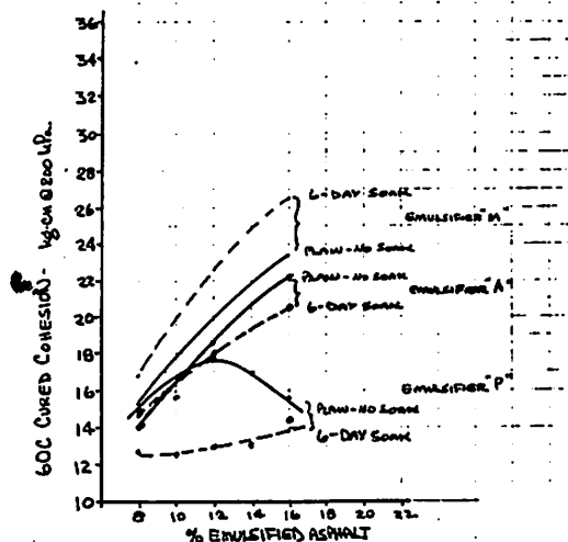
EXAMPLE 8. EFFECT OF 6-DAY SOAK ON 60C CURED COHESION
