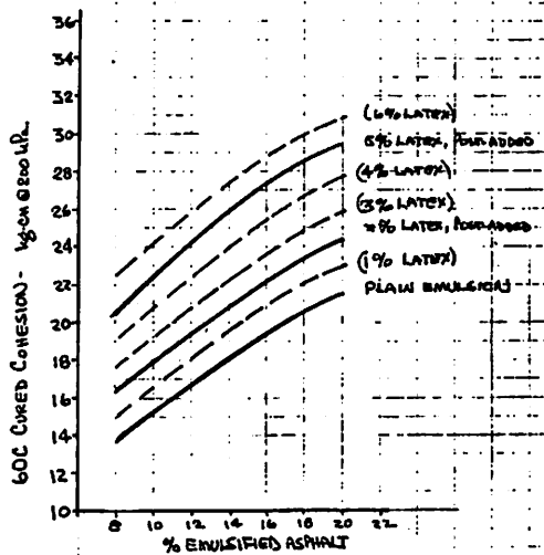
EXAMPLE 4. EFFECT OF LATEX POST-ADDITION
