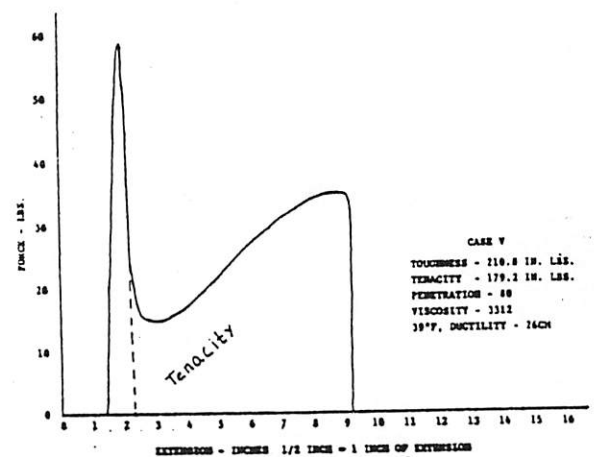
FIGURE 5. TOUGHNESS AND TENACITY CURVES FROM REINKE & O'CONNELL.
