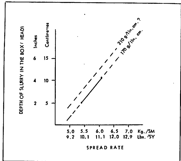
Figure 11. EFFECT OF SLURRY DEPTH ("HEAD") ON THE SPREAD RATE (Median Type 2 Slurry-- 2.5 cm. Consistency-- 170 g/l in. cm. sludge contact pressure-- applied to a smooth surface.)
