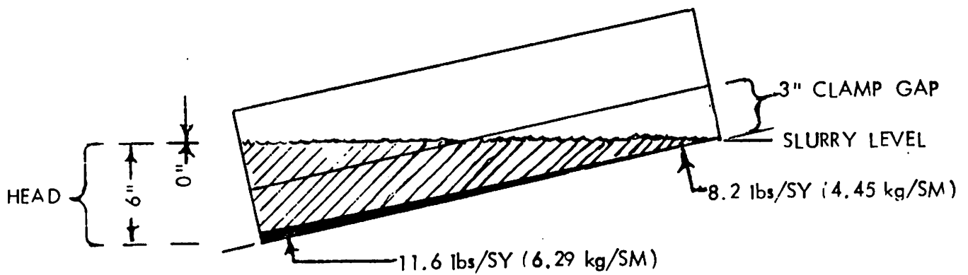
10% SUPERELEVATION SECTION - 40% VARIATION
