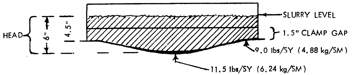
1.5" RUT SECTION - 30% VARIATION
