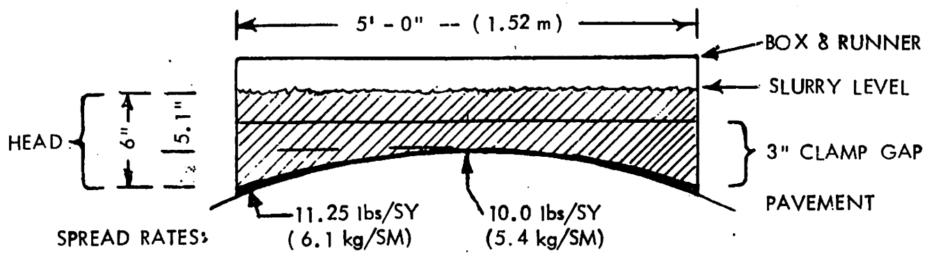
3% CROWN SECTION - 12% VARIATION
